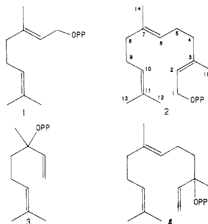
Scheme II Cyclization of Farnesyl Pyrophosphate
