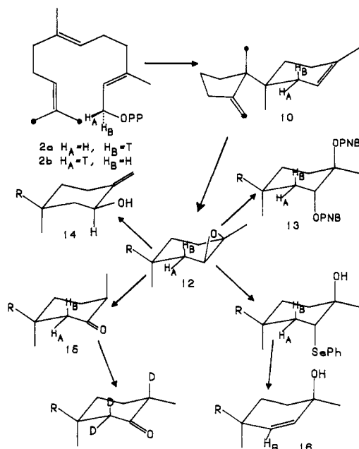
Scheme X Degradation of Trichodiene Derived from (1 R )-[1- 3 H,12,13- 14 C] Farnesyl Pyrophosphate and (1 S )-[1- 3 H,12,13- 14 C] Farnesyl Pyrophosphate To Establish the Stereochemistry of Labeling at C-11
