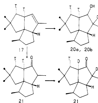
Scheme XIII Degradation of Pentalene Derived from [9- 3 H 2 ,12,13- 14 C] Farnesyl Pyrophosphate and Location of Half the Tritium Label at C-8
