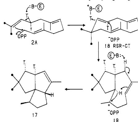
Scheme XIII Degradation of Pentalene Derived from [9- 3 H 2 ,12,13- 14 C] Farnesyl Pyrophosphate and Location of Half the Tritium Label at C-8
