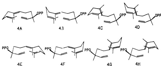
Scheme IX Cyclization of (1 R )-[1- 3 H,12,13- 14 C] Farnesyl Pyrophosphate (2a) and (1 S )-[1- 3 H,12,13- 14 C] Farnesyl Pyrophosphate (2b) to Trichodiene (10) by Way of Conformer 4A of Nerolidyl Pyrophosphate and the Bisaboly Cation 11 with Retention of Configuration at C-1
