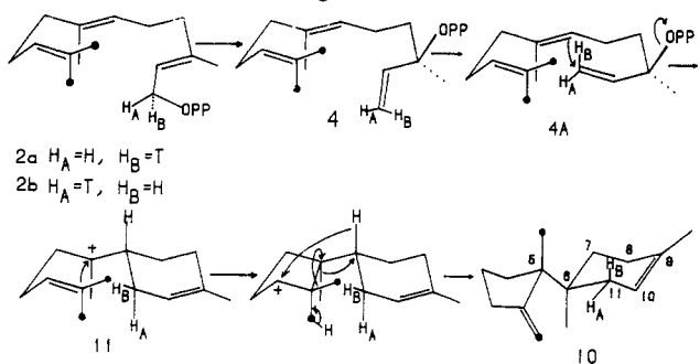
Scheme IX Cyclization of (1 R )-[1- 3 H,12,13- 14 C] Farnesyl Pyrophosphate (2a) and (1 S )-[1- 3 H,12,13- 14 C] Farnesyl Pyrophosphate (2b) to Trichodiene (10) by Way of Conformer 4A of Nerolidyl Pyrophosphate and the Bisaboly Cation 11 with Retention of Configuration at C-1
